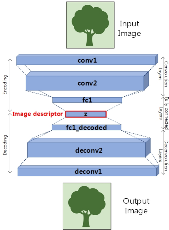
[Fig. 2] The structure of the proposed CAE. This structure is divided into the encoding and the decoding parts. The first part transforms an input image to a low dimensional latent representation, and the second part reconstructs it to the input image
