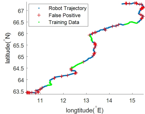
[Fig. 6] The place recognition results of the robot trajectory. The blue line is the robot trajectory, and the green dots are the locations of the training data. Locations marked with a red cross are false positives
