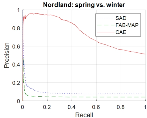
[Fig. 5] The comparison of the precision-recall curve results of the Nordland spring-winter dataset. The results showed that our method outperforms than other methods
