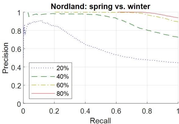
[Fig. 4] Precision-recall curve results of the Nordland spring-winter dataset. The higher the ratio of the training data, the better the performance of the place recognition
