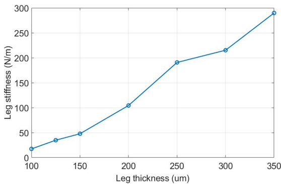
[Fig. 11] Relationship between leg stiffness and leg thickness
