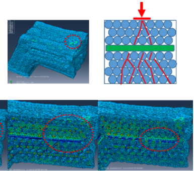
[Fig. 6] FEM simulation with backbone
