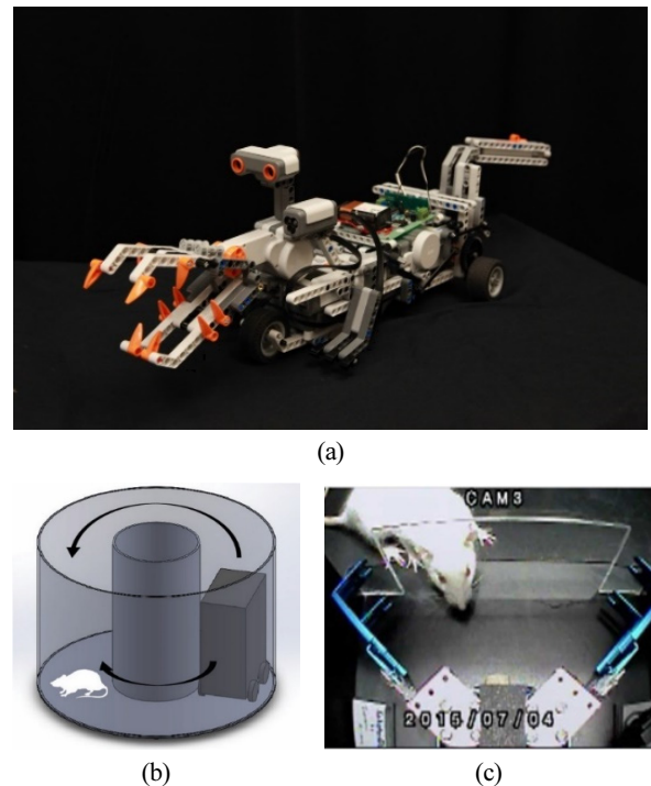
[Fig. 2] Examples of simple robots used in rat studies; (a) An alligator-shaped predator robot [13] , (b) A box-shaped chasing robot [29] , (c) Lobster-bot: A biting robot [30]
